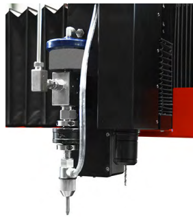
Equipment for pre-drilling of fragile and multi-laminated composites. Possible to mount different drill bit diameters.
