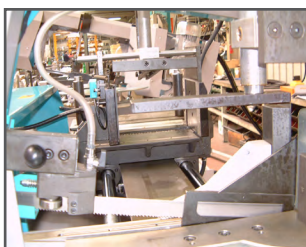
Hydr. device for bundle cutting
