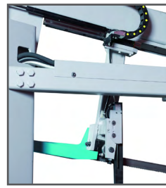
Mobile blade guide automatically kept in contact with the cutting point.
