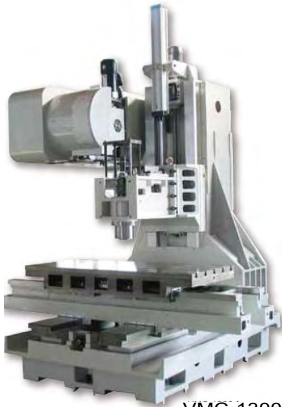
VMC-1300 frame
