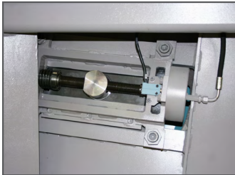
Blade tensioning KTECH via electro-mechanical system, CNC-controlled
