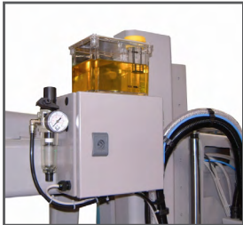
Minimal lubrication
