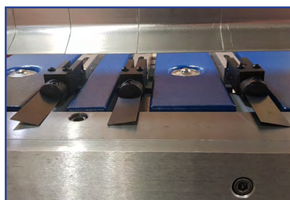
Solid lower beam tool and feather grooves
