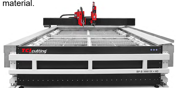
BP-S (Standard) 3060
