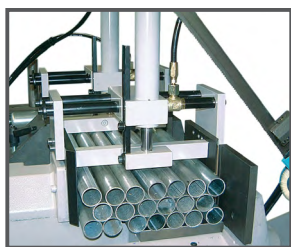
Bundle cutting
