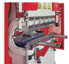
Laser protection
