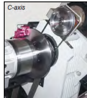
C-axis with braking system provides spindle angle indexing & superior performance
