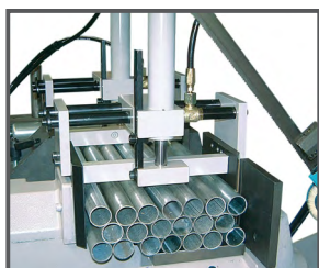
Bundle cutting
