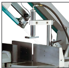
Hydraulic vertical vice
