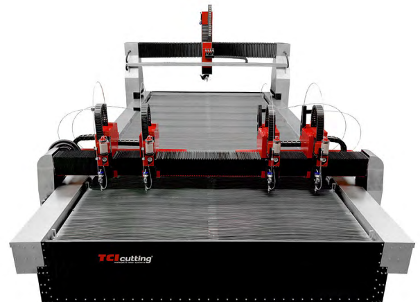
BP-M (Modular) 4060
