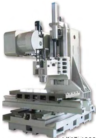
VMC-1300 stativ
